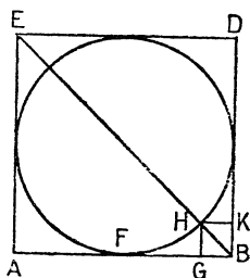
FIG. 8.—ANOTHER METHOD OF FINDING \sqrt{2} .
